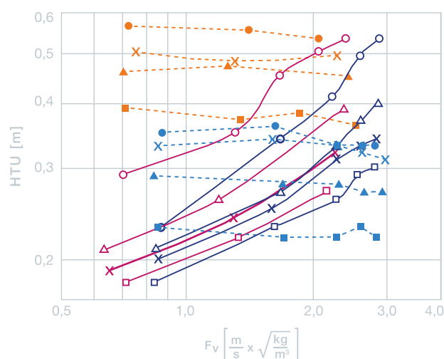
HTU: VFF-Twin-Pak® No. 2 vs. Pall-50-M
